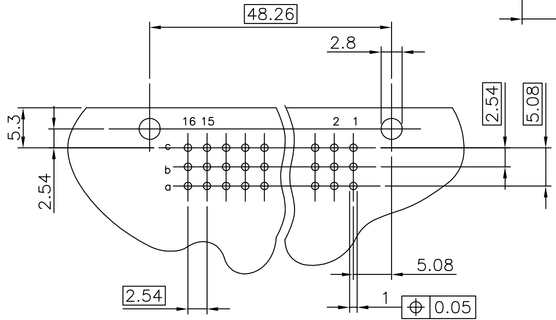
P.C. MOUNTING HOLE PATTERN
